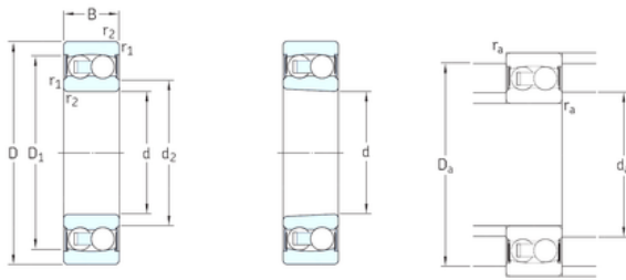
Cylindrical bore
